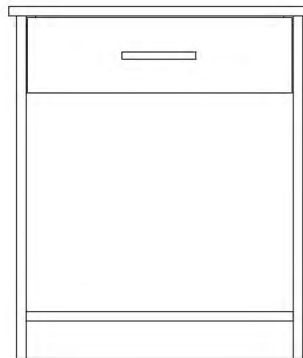
SM-P104A Nightstand 24" w x 16" d x 28" h
