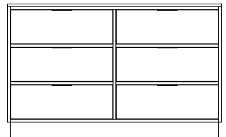
TV Dresser Bedroom GST-308-CSG 54"W x 24"D x 34"H
