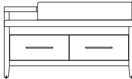
LUGGAGE BENCH WITH DRAWER CS-LB-DRAWER 48"W x 24"D x 27 1/2"H
