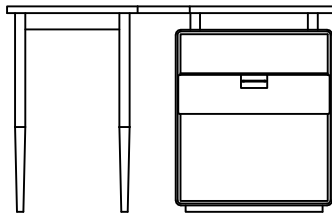
Desk with Nightstand (K/D) 68"W x 50"D x 31 1/2"H
