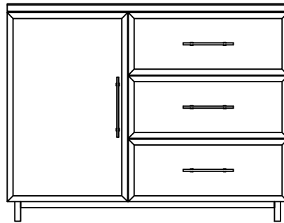
Combo 56"W x 24"D x 43 1/2"H
