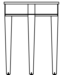
SIDE TABLE CIS-SIDE-T 20"DIA x 26"H
