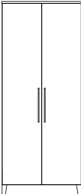
ADA WARDROBE CIS-WARDROBE-ADA 32 1/4"W x 24"D x 78"H
