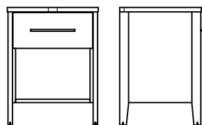
20" NIGHTSTAND-WITH GROMMET SMALL NS-CS-20 20"W x 18"D x 26"H
