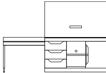
Streamline Desk Unit No Refrigerator ADS Compliant GR-323 105"W x 24"D x 71"H
