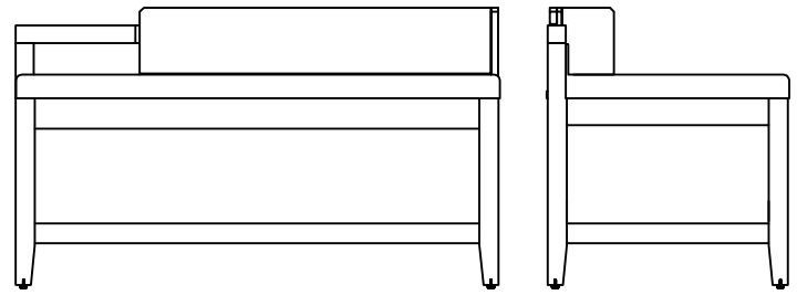
LUGGAGE BENCH NO DRAWER CS-LB 48"W x 24"D x 27 1/2"H
