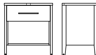
24" NIGHTSTAND-WITH GROMMET LARGE NS-CS-24 24"W x 18"D x 26"H
