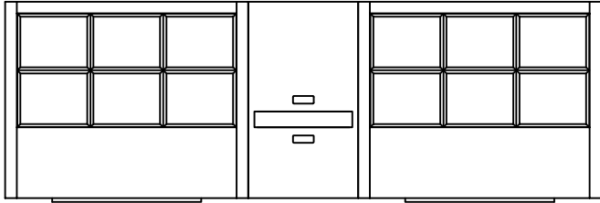
Queen Headboard Option A (K/D) GR-302.A 152"W x 3"D x 50"H
