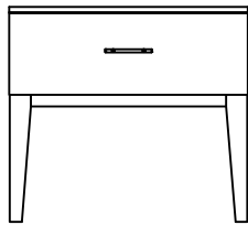
30" Nightstand 30"W x 20"D x 27"H
