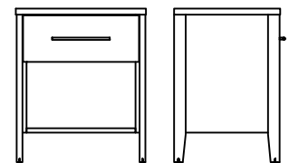
22" NIGHTSTAND-NO GROMMET SMALL NS-CI-22 22"W x 18"D x 26"H
