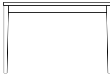
Desk 48"W x 24"D x 31 1/2"H
