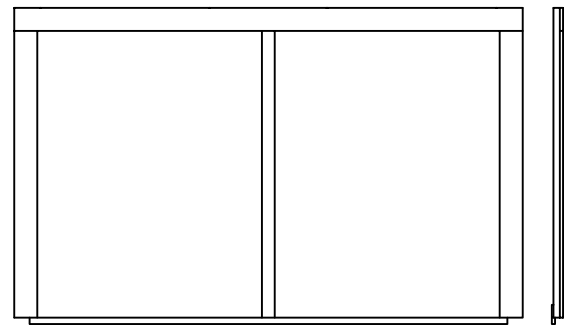
KING HEADBOARD SHORT CI-KH-SHORT 78"W x 1 1/2"D x 47 1/2"H
