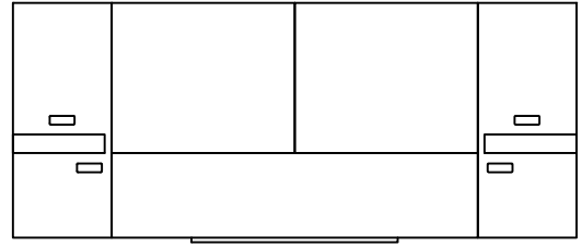
King Headboard Option B (K/D) GR-301.B 120"W x 3"D x 50"H
